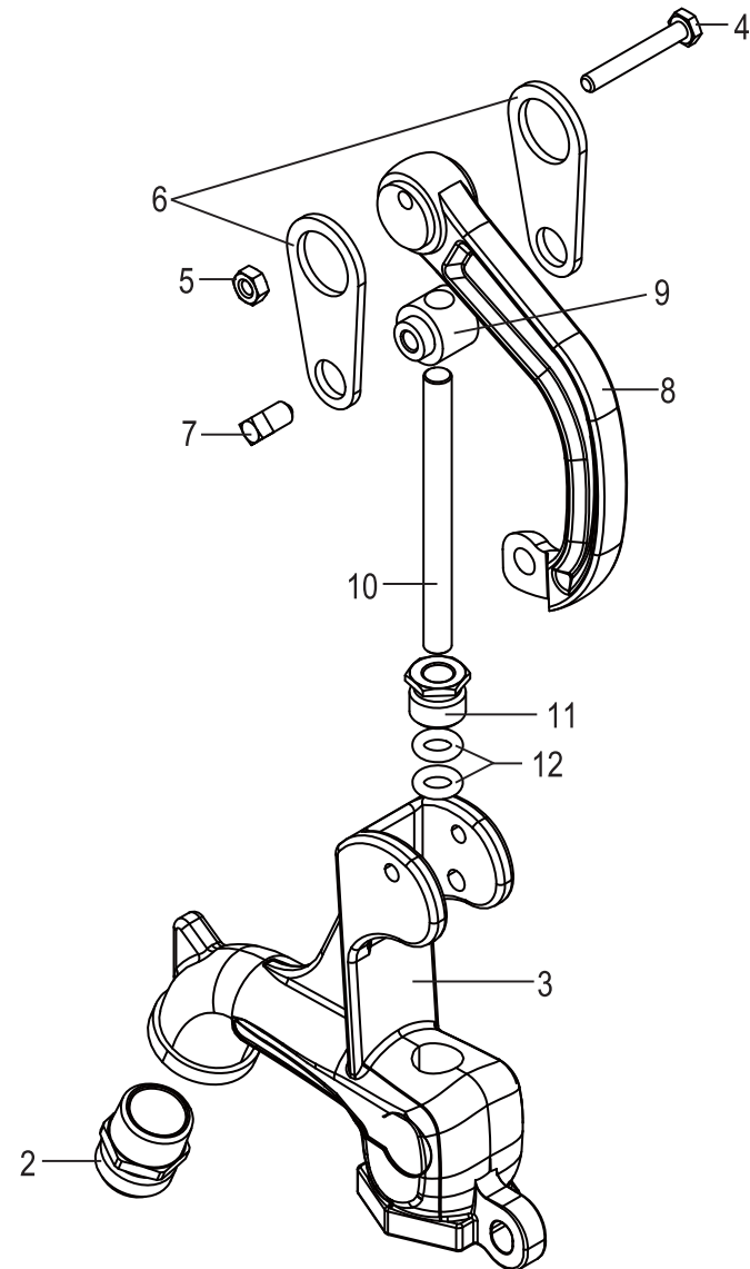
YHC-BLUE & YHHD-BLUE Exploded View
